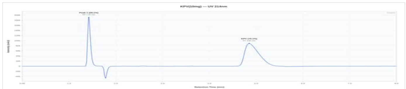
KPV 10mg - KP1026232JP: UV Chromatogram
