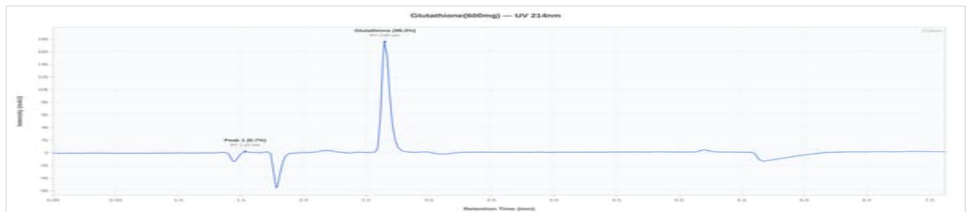
Glutathione 600mg - GT60026232JP: UV Chromatogram
