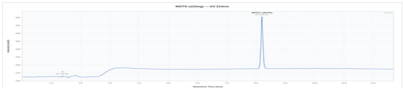
MOTS-C 10mg - MC1026233GX: UV Chromatogram
