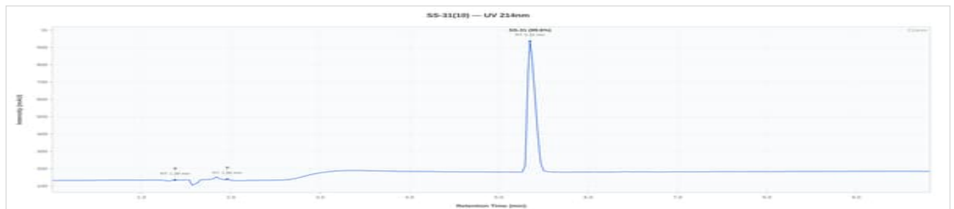
SS-31 10mg - SS1026233GX: UV Chromatogram
