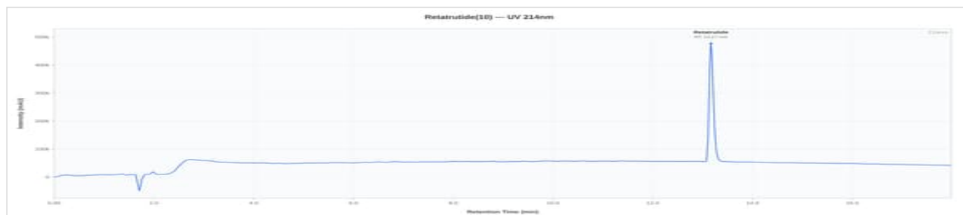
Retatrutide 10 - RT1026258JP: UV Chromatogram
